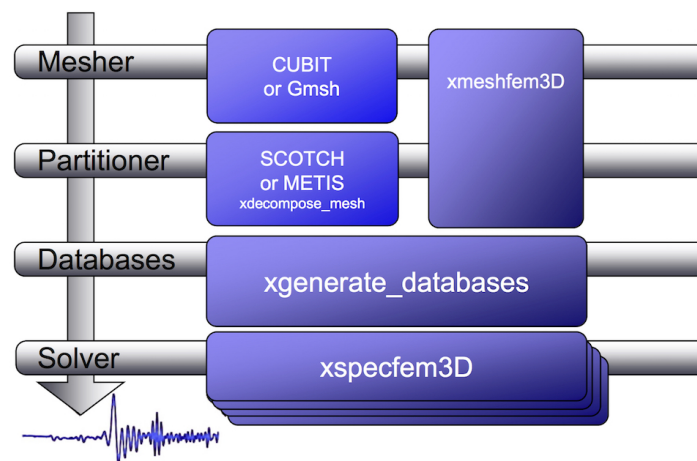
Figure 4.1: Schematic workflow for a SPECSEM3D Cartesian simulation. The executable xgenerate_databases creates the GLL mesh points and assigns specific model parameters.
